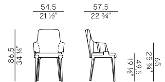
942/PB7W poltroncina dining schienale alto \ high backrest dining armchair
