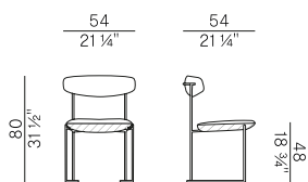
922/MB sedia dining \ dining chair
