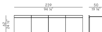
884/MB2 madia \ sideboard
